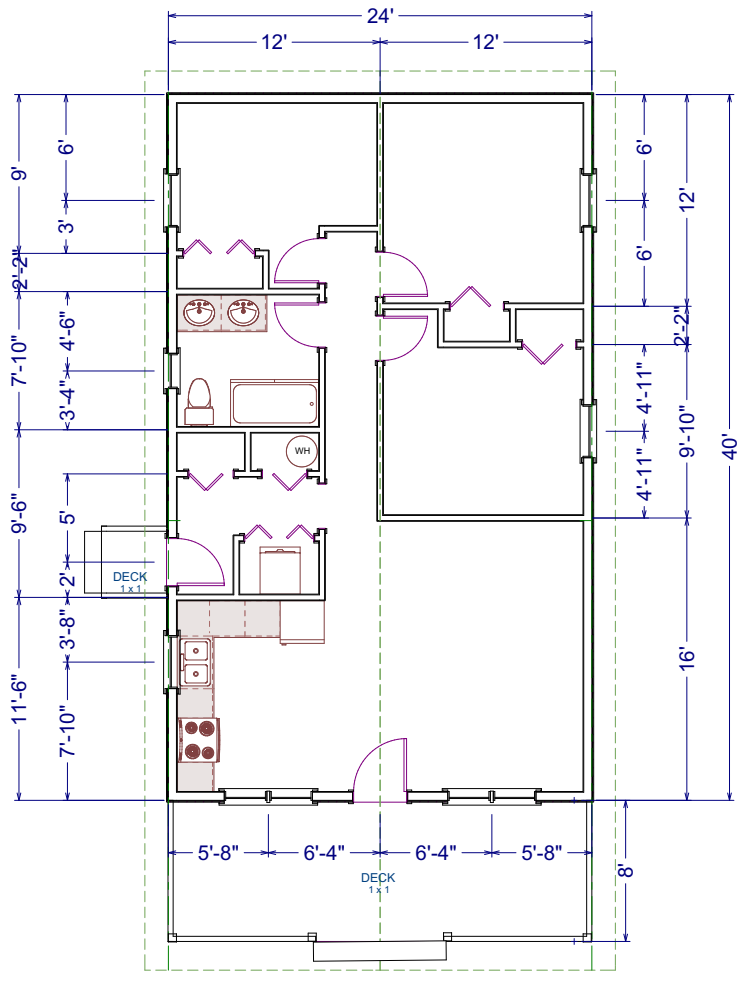
LIVING AREA 960 sq ft
